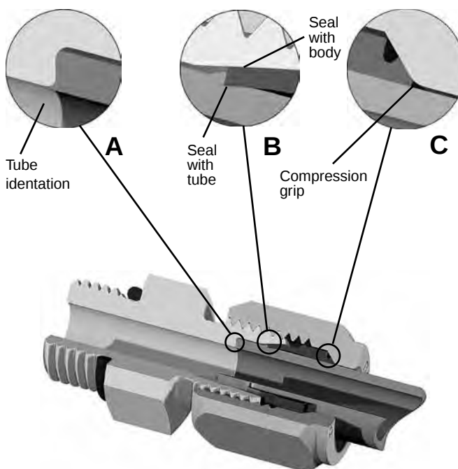
Fig. C1 – Assembled Ferulok Fitting with Tube
