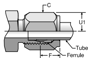
Ferulok Tube End Assembly
